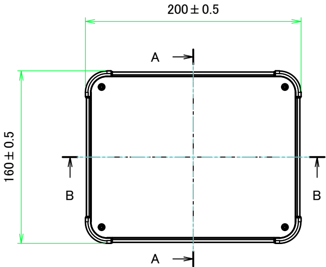
E view
